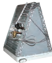
Model CAPVU Vertical Uncased A-Coil
