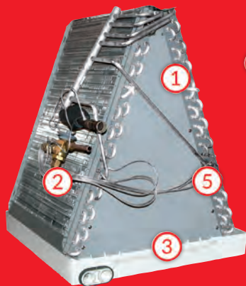
Model CAPVU Vertical Uncased A-Coil
