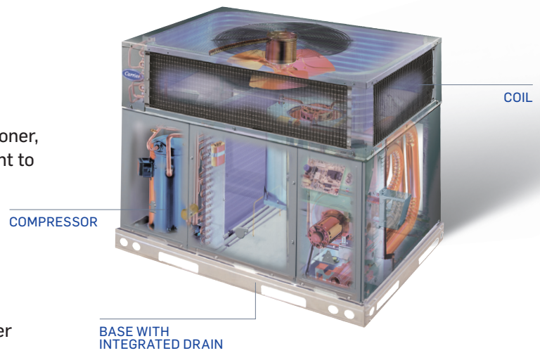
PACKAGED GAS FURNACE/AIR CONDITIONER SHOWN
