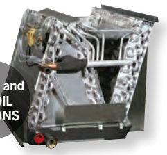
Aluminum Evaporator Coils
