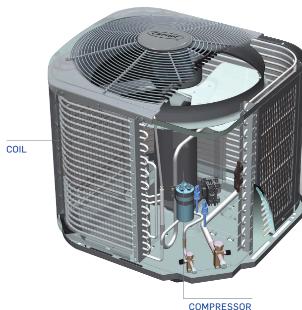
PERFORMANCE™ SERIES AIR CONDITIONER
