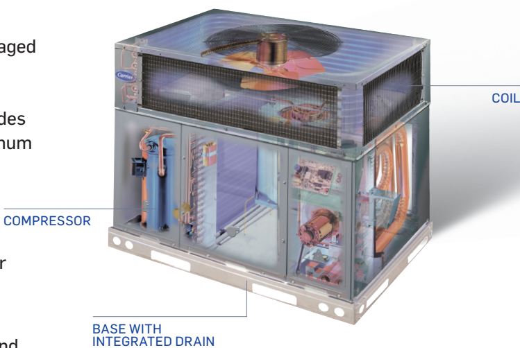
PACKAGED GAS FURNACE/ AIR CONDITIONER SHOWN
