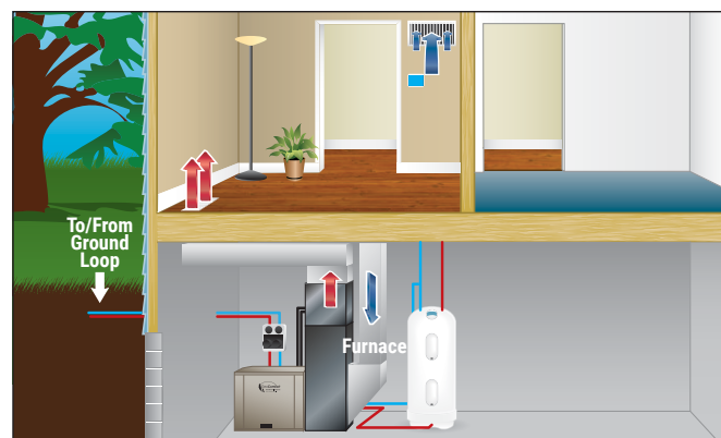
Common hybrid heating system with furnace.
