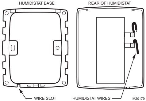
Fig. 13. Humidistat base and rear view.
