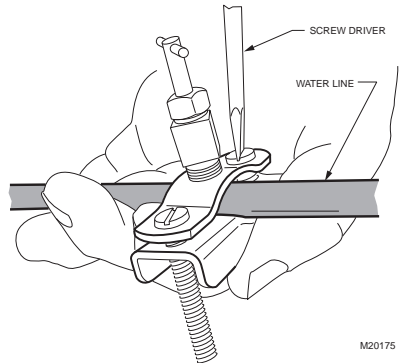
Fig. 8. Installing the saddle valve.
