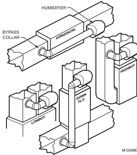
Fig. 1. Typical humidifier installation locations.
