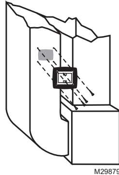
Fig. 15. Secure the base bracket to the duct.
