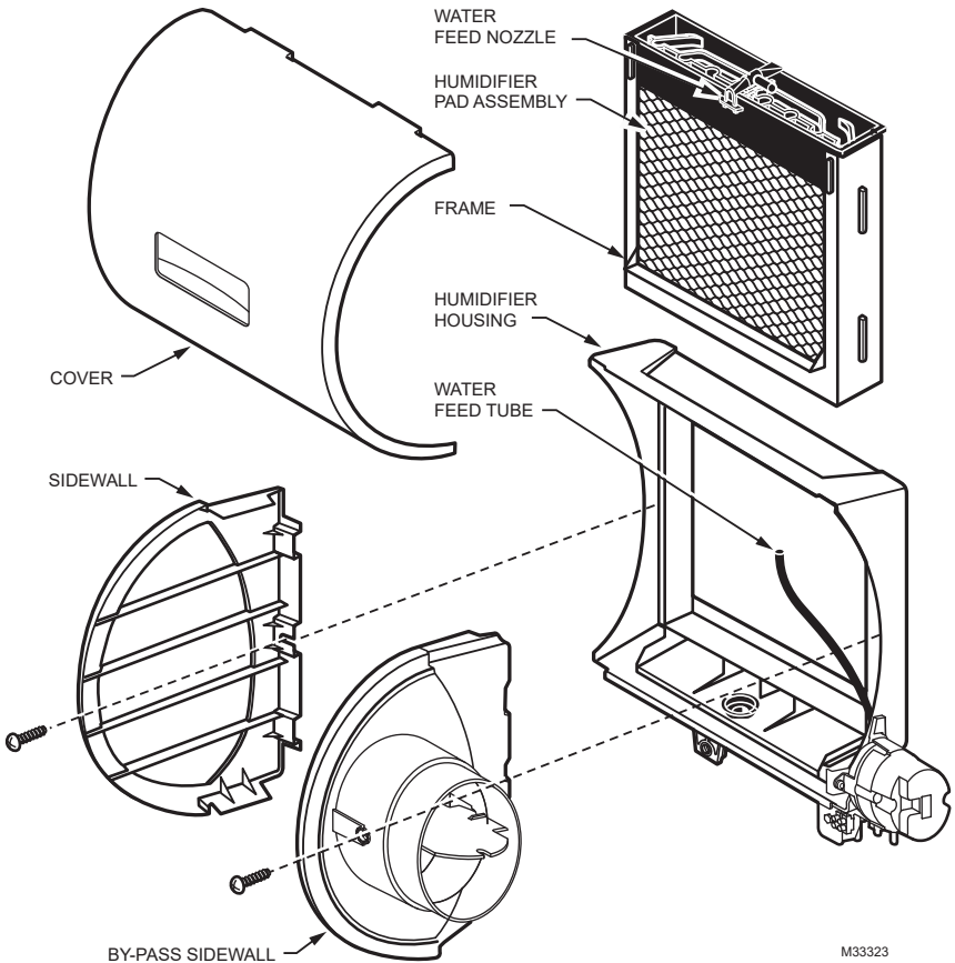
Fig. 4. Disassembling humidifier.
