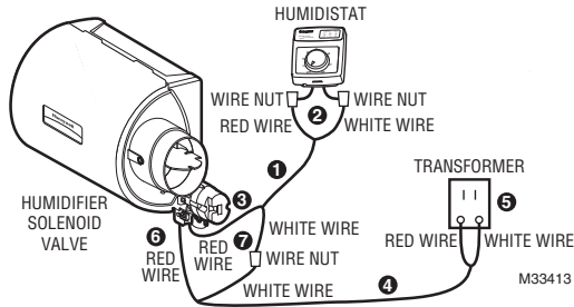
Fig. 16. Wiring the controls and the HE240.
