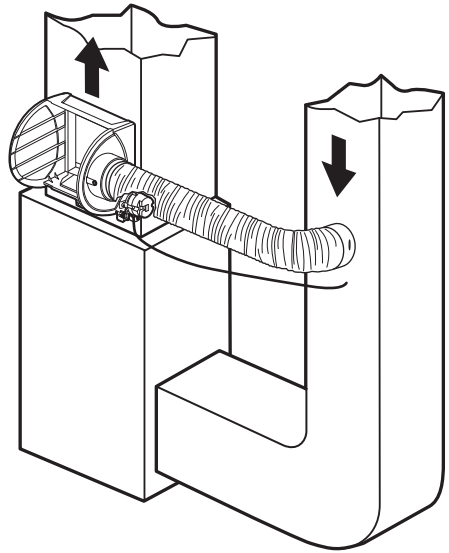
Fig. 12. Installing the pressure switch tubing.
