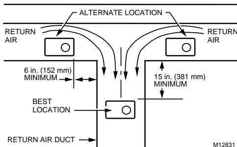
Fig. 3. Selecting duct location for humidistat.
