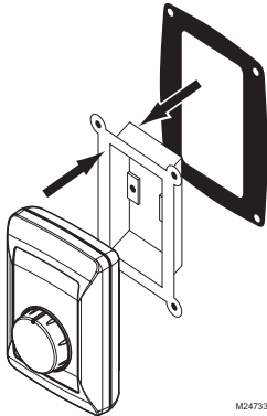
Fig. 14. Slide the foam gasket onto the base.
