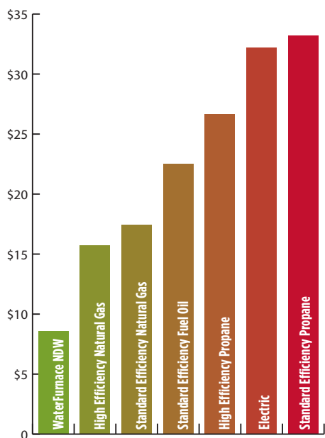
Cost per million BTUs of hot water
