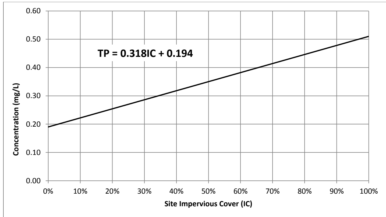
Figure 11-14 Average Concentration of Total Phosphorus in Stormwater Runoff
