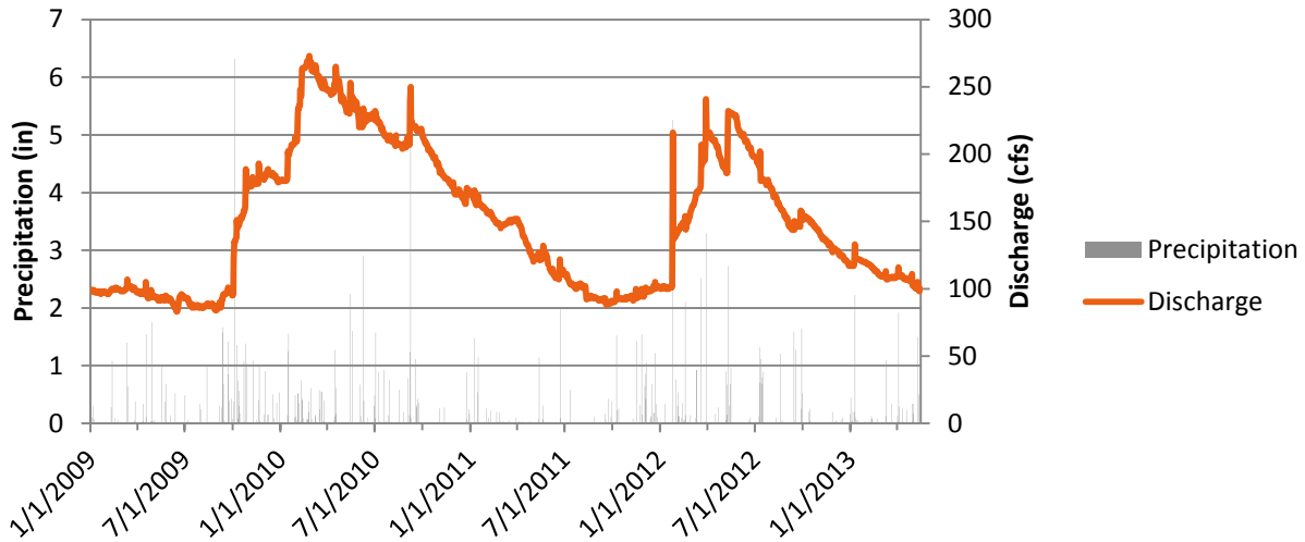
Figure 9. Discharge and precipitation data for San Marcos between January 2009 to May 2013.
