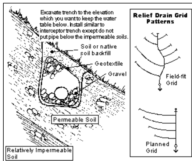
Figure 10-1: Relief Drain Example from Washington Dept. of Ecology
