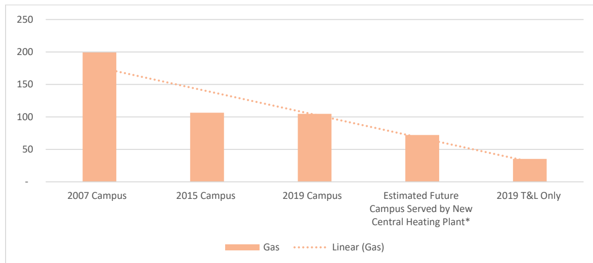
Figure 15: Natural Gas Use Intensity Trend Comparison Campus vs. T & L Building
