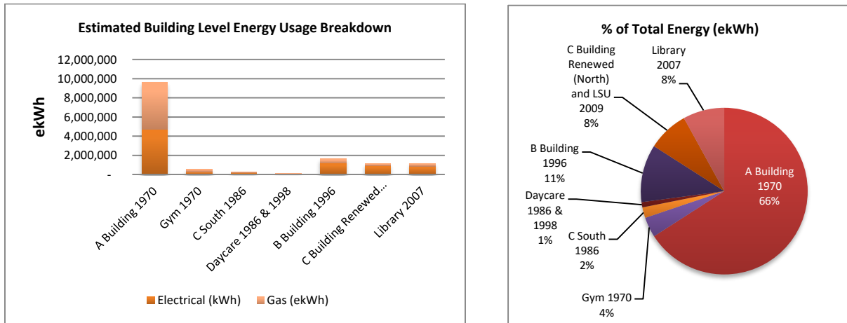
Figure 10: Buildings energy usage breakdown 2015 Estimate
