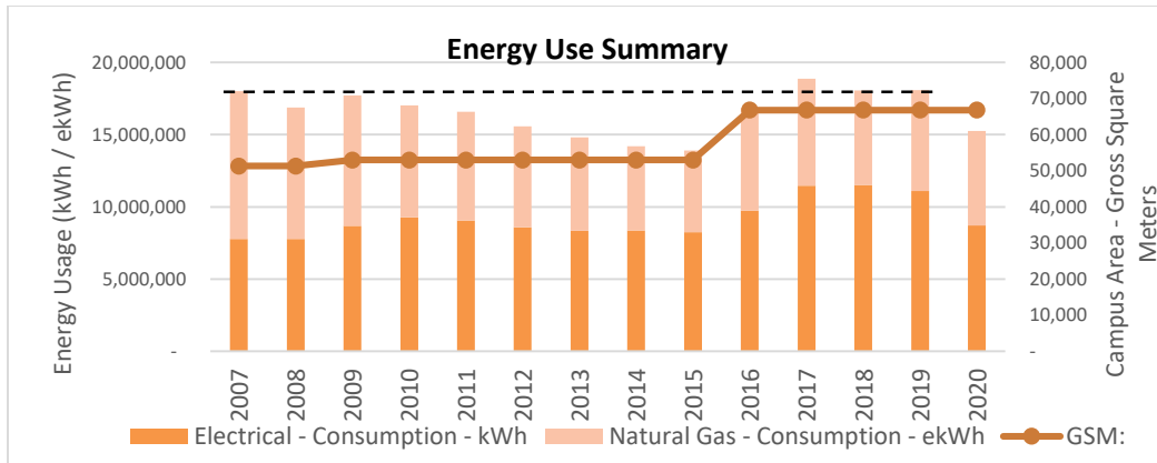
Figure 3: Energy Use Summary Chart
