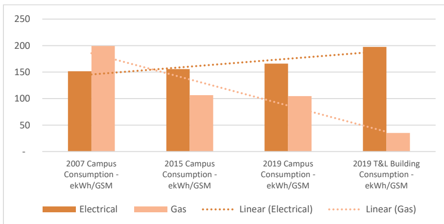
Figure 14: Energy Use Intensity Trend Comparison 2020 Analysis Campus versus T & L Building
