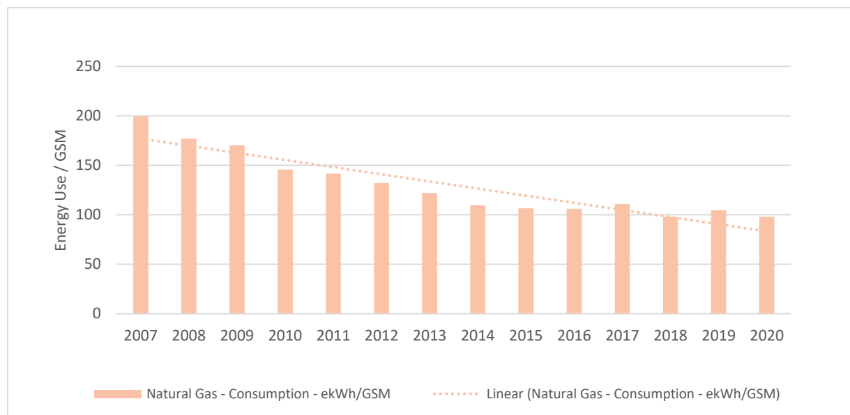
Figure 7: Natural Gas Usage per GSM Trend
