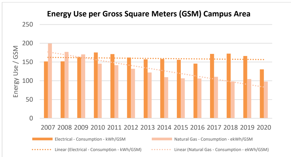
Figure 6: Energy Use per GSM by Energy Type Trend
