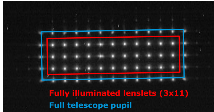
Figure 3. M2MM overview (left) and WFS sample pattern (right). The M2MM provides five degrees of freedom (three translations and two rotations) control over the Gaia telescope secondary mirrors. They are only operated during the rare refocusing events. Image: Airbus DS. Two Shack-Hartmann WaveFront Sensors (WFS) provide low-order sampling needed during the first focusing attempts in early commissioning and differential measurements for fine tuning during the nominal mission.
