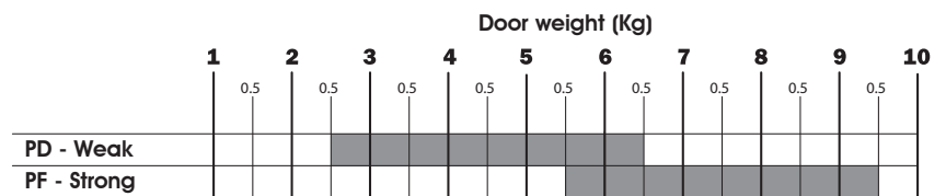
CHART TO SELECT THE EXACT SYSTEM SUITABLE FOR THE DIMENSIONS AND WEIGHT OF THE DOOR.
