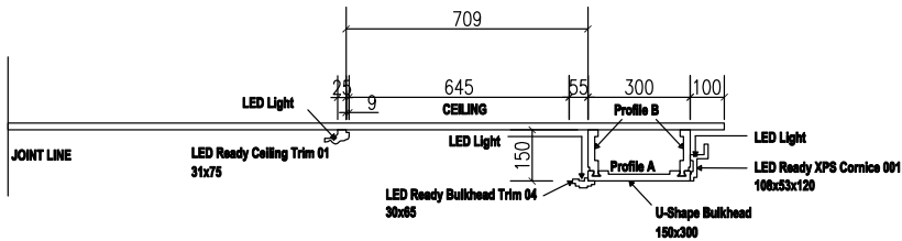
CEILING SECTION
