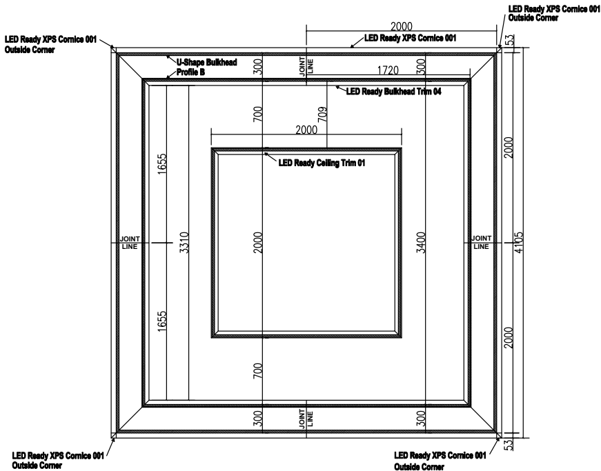
CEILING PLAN
