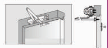
C Parallel rocking arm pedestal install
