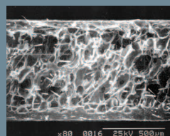
Scanning electron microscope image of Aerated Poly Cone showing air pockets.
