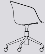
AAC 53 UPHOLSTERY W69 x D69 x H74,5-87,5/ SH42,4-55,4 cm
