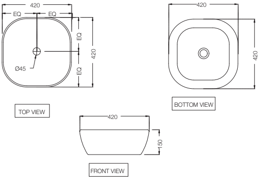
JDS-BLM-25911 R 1846 Thin Rim Table Top Basin In Black Matt, Size: 420x420x150 mm, Shape - Square
