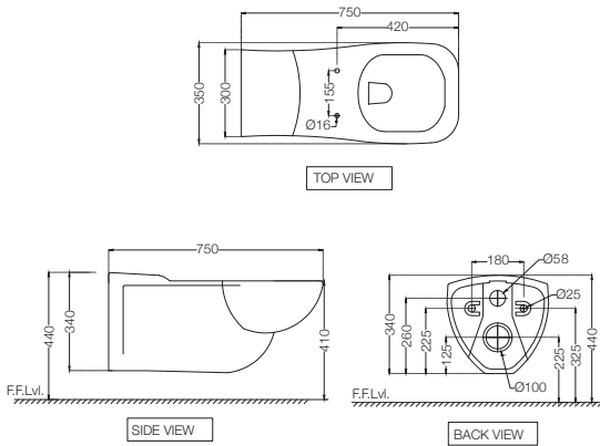
DIS-WHT-93951UF R 7943 Wall Hung WC With UF Soft Close Seat Cover, Hinges And Accessories Set, Size: 350x750x340 mm
