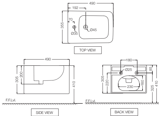
KUS-WHT-35153 R 4014 Blind Installation Wall Hung Bidet With Accessories Set, Size: 355x490x305 mm
