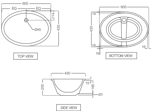
CNS-WHT-705 Under Counter Basin With Fixing Accessories, Size: 605x430x200 mm, Shape: Oval R 937
