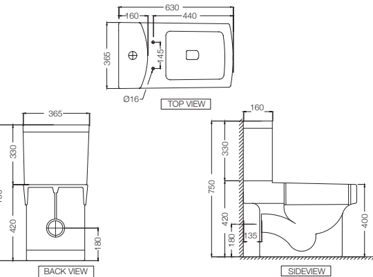
FNS-WHT-40751P180UFMSZ R 5038 Bowl With Cistern For Coupled WC With UF Soft Close Slim Seat Cover, Hinges, Dual Flush Cistern Fitting And Fixing Accessories, Size: 365x630x750 mm, P Trap-180 mm
