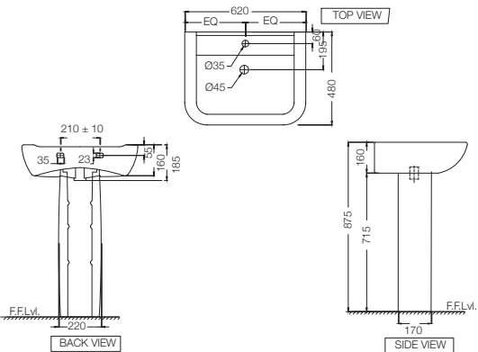
FNS-WHT-40801 R 1251 "Wall Hung Basin With Fixing Accessories, Size: 620x480x185 mm" FNS-WHT-40301 R 779 Full Pedestal For FNS-WHT-40801
