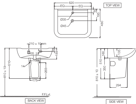
FNS-WHT-40801 R 1251 "Wall Hung Basin With Fixing Accessories, Size: 620x480x185 mm" FNS-WHT-40305 R 551 Half Pedestal With Fixing Accessories For FNS-WHT-40801
