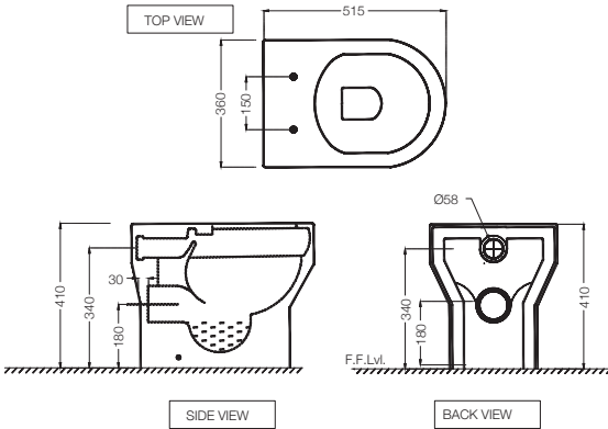
DIS-WHT-93955P180UF R 4872 Rimless Back To Wall WC With UF Soft Close Seat Cover, Hinges, Fixing Accessories And Accessories Set, Size: 360x515x410 mm, P Trap- 180 mm
