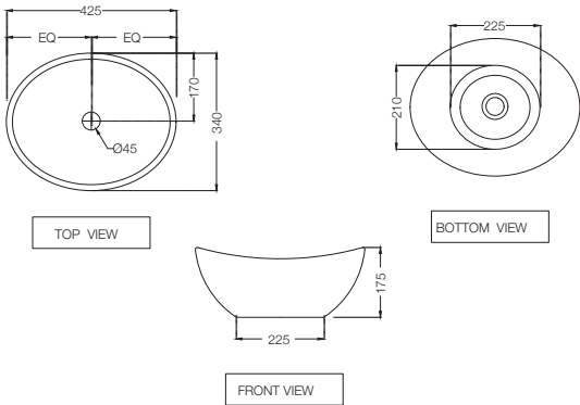
CNS-WHT-903 Table Top Basin, Size: 425x340x175 mm R 742
