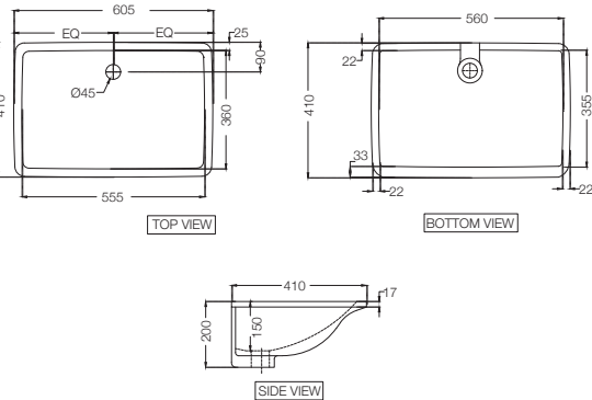
FNS-WHT-40701 R 1077 Under Counter Basin With Fixing Accessories, Size: 605x410x200 mm, Shape: Rectangular
