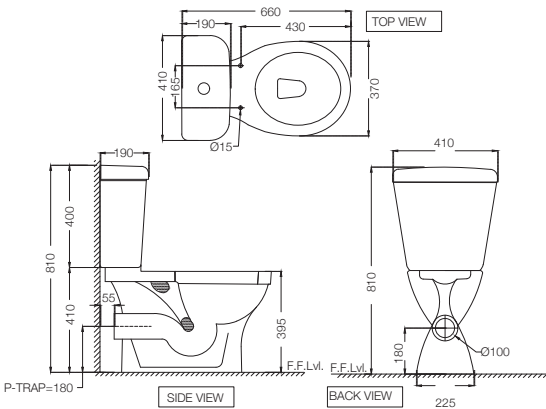
CNS-WHT-751P180SPPZ Bowl With Cistern For Coupled WC With PP Soft Close Seat Cover, Hinges, Dual Flush Cistern Fitting, Fixing Accessories And Accessories Set, Size: 410x660x810 mm, P Trap- 180 mm R 1899
