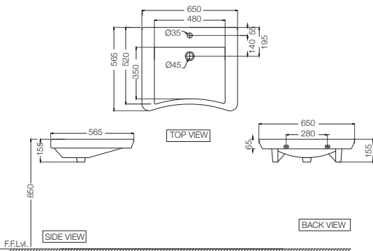
DIS-WHT-93801 R 3050 Wall Hung Basin With Fixing Accessories, Size: 650X565X155 mm
