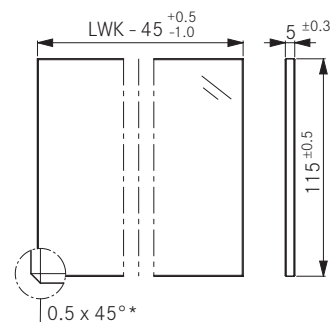
Cutting dimensions of front glass inlay
