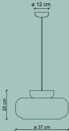
art. C2741 peso netto / net weight Kg 2,90 1 x MAX 53W E27
