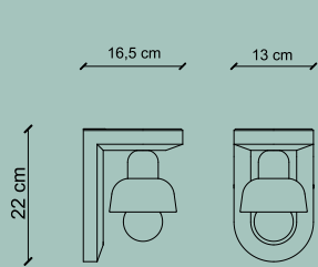
art. C2600 peso netto / net weight Kg 1,14 1 x MAX 28W E27
