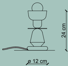
art. C2604 peso netto / net weight Kg 1,14 1 x MAX 53W E27
