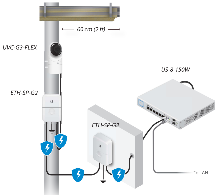
Diagram Showing Use of Ethernet Surge Protectors
