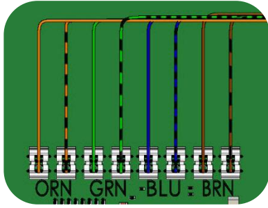
DETAIL G 8-WIRE ETHERNET CONNECTION
