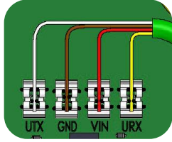
DETAIL H 4-WIRE CONNECTION
