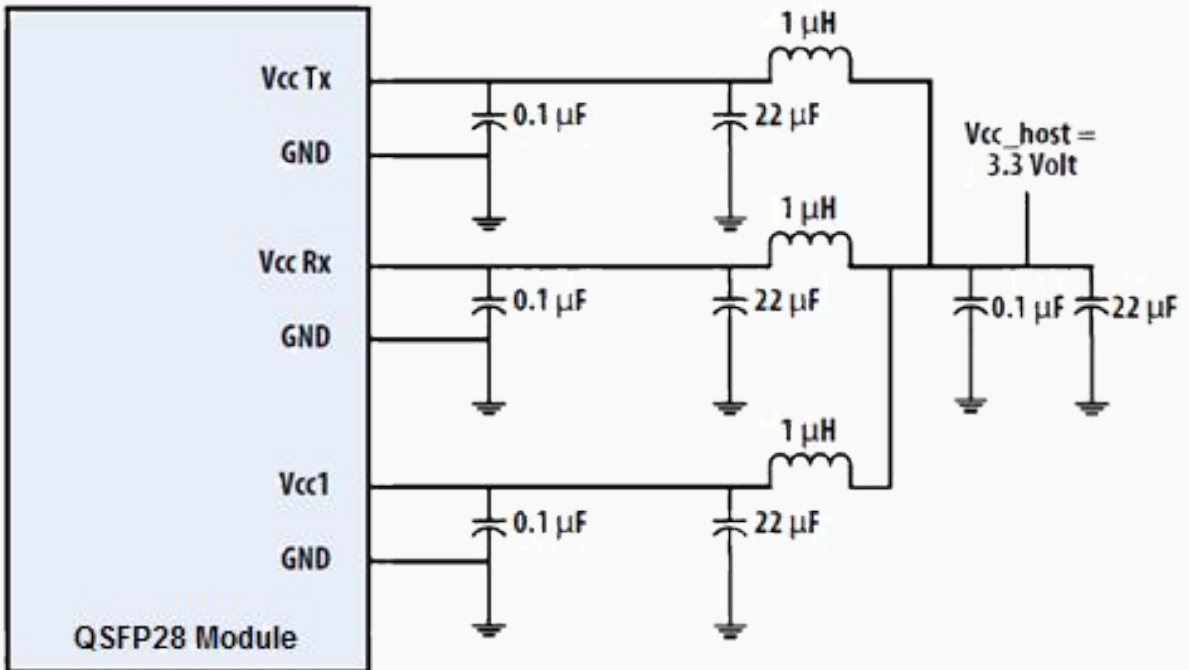
Figure 4. Recommended Power Supply Filter
