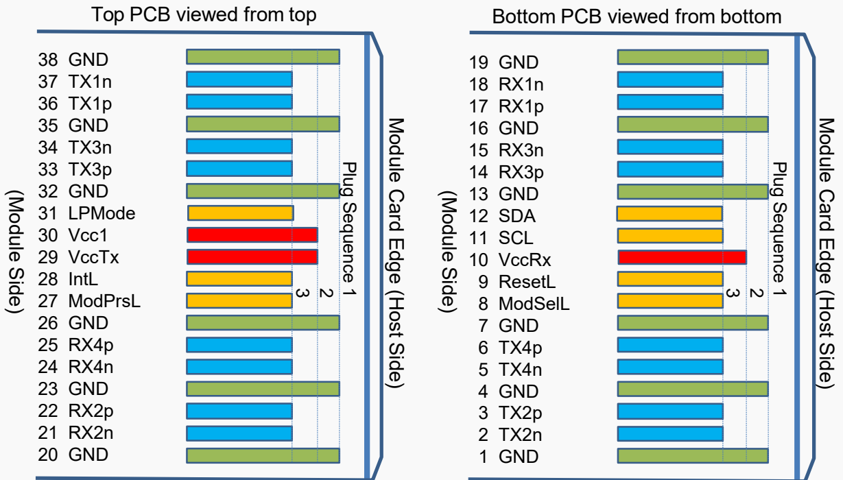
Figure 2. MSA Compliant Connector
