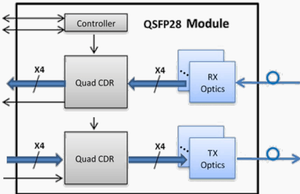
Figure 1. Transceiver Block Diagram
