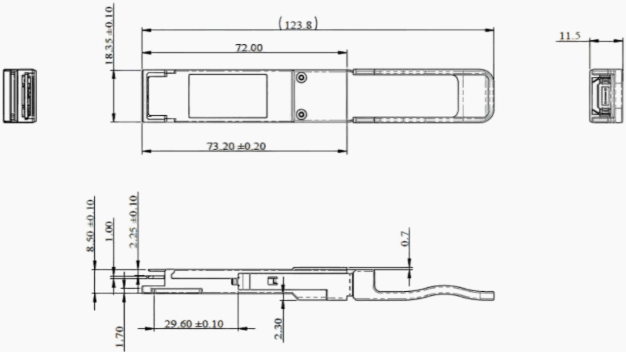
Figure 5. Mechanical Outline
