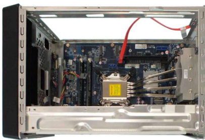
Shuttle XPC Cube Barebone SH510R4 (Photo without chassis cover)
