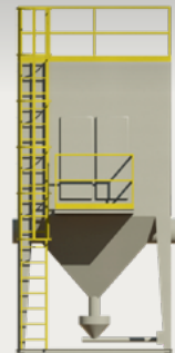
Dimensions: 24'6" x 11' x 8'3" Weight: 9,200 Lbs
