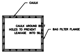
TYP. CAULKING DETAIL
