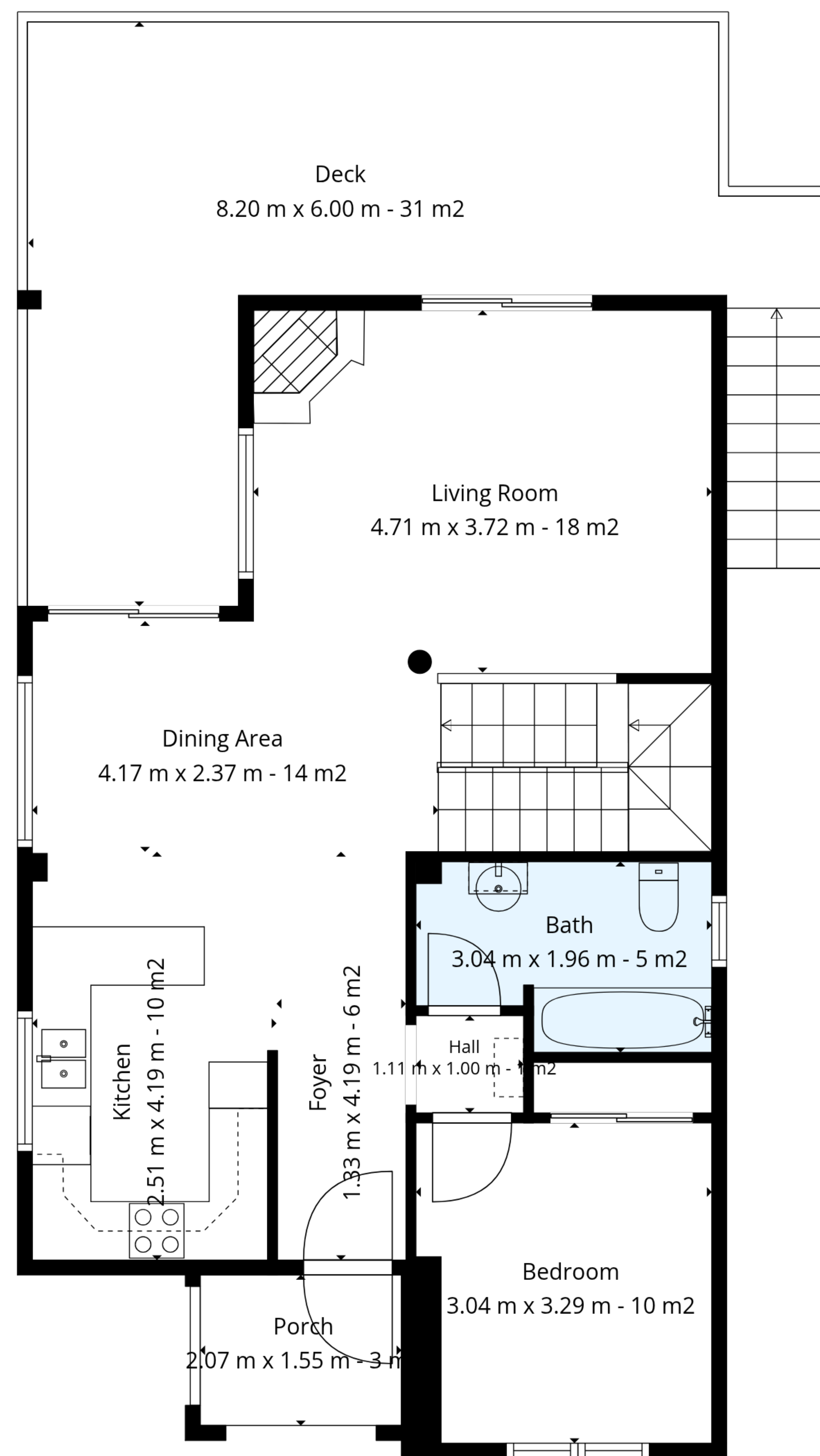
2nd Floor
