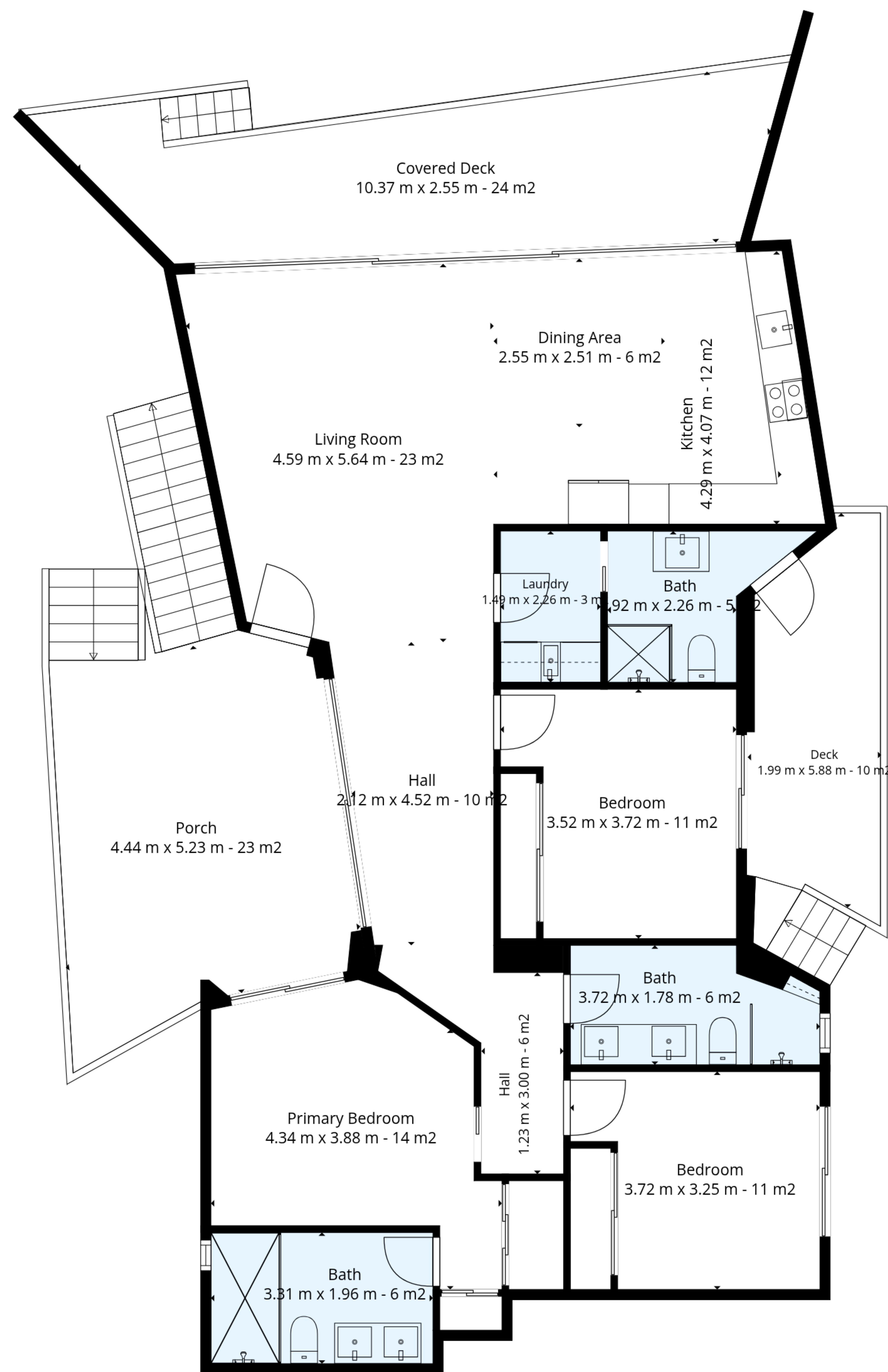
1st Floor
