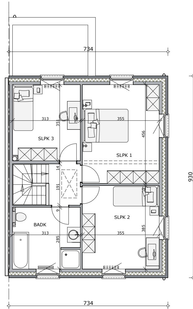
VERDIEPING Opp.= 68.26 m 2
