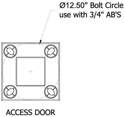
6" Anchor Base
