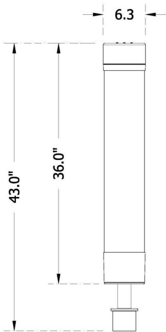
Slip Fit Mount (SF_)
