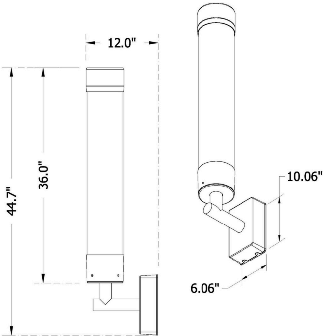
Wall Mount (1W)
