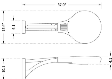
Wall mounted "F01S" arm (1W-F01S)
