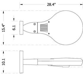
Wall Mount with a Flat Mount Adapter (1W-FMA)
