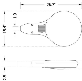
Flat Mount Adapter or Round Pole Adapter (FMA/RP345)
