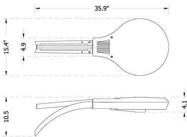
Pole mounted "F01S" arm (F01S)
