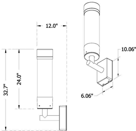
Wall Mount (1W)
