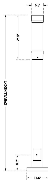
WIDE BASE FOR HEIGHTS > 12'
