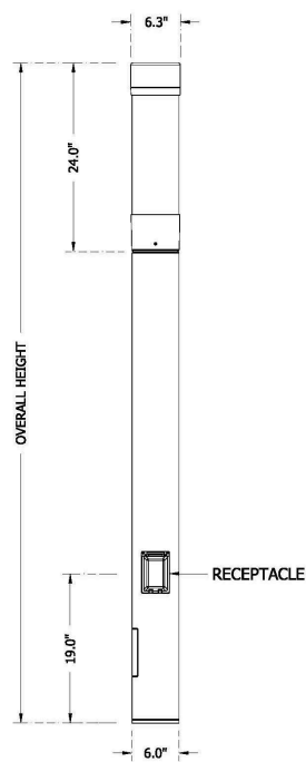
LOW-PROFILE BASE FOR HEIGHTS ≤ 12'
