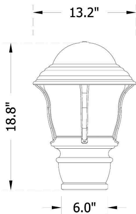
Full Body Lens, 5" Slipfitter (E260LED-R5)
