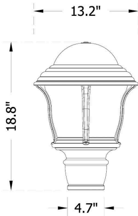
Full Body Lens, 4" Slipfitter (E260LED-R4)
