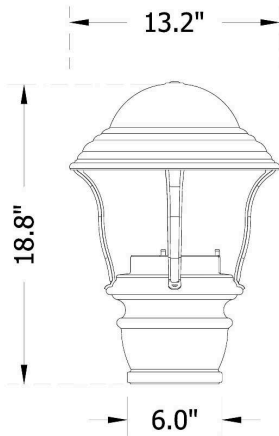
Open Body, 5" Slipfitter (E250LED-R5)
