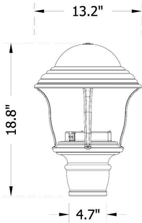
Open Body, 4" Slipfitter (E250LED-R4)
