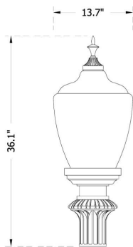
With Finial, "7_" Fitter (B740CF-7_)
