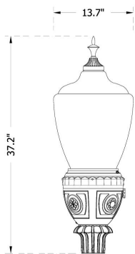
With Finial, "992T" Fitter (B740CF-992T)
