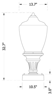
No Finial, "5P" Fitter, Pier Base (450PB-B740-5P)
