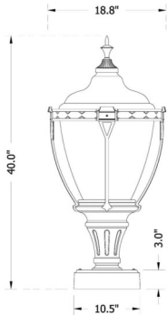
"5P" Fitter, with finial, Pier Base (450PB-B780-5P)
