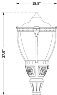
"990" Fitter, No finial (B780NF-990)
