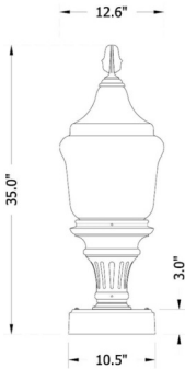
Pier Base (450PB-D640-5P)
