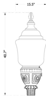
Solid Roof, "992T" Fitter (D650SR-992T)
