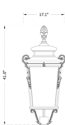
Large Venice Post Top (V410)
