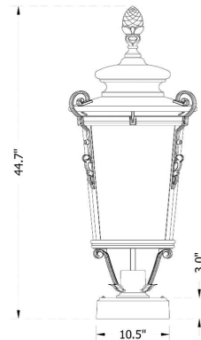
Pier Mount (450PB-V410)
