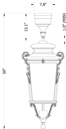
Stem or Chain Hung (SH28/CH28-V410)
