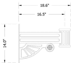
TA-SCR (Wall/Side Mount, Scroll Arm)
