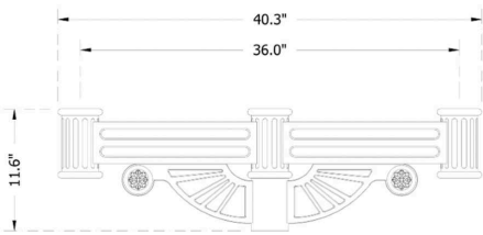
2-TA-SCR / 4-TA-SCR (Post Top, Double / Quad, Scroll)
