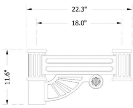
1-TA-SCR (Post Top, Single, Scroll Arm)
