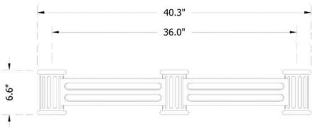
2-TA-SCR / 4-TA-SCR (Post Top, Double / Quad, Scroll)
