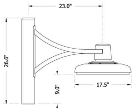
Sweep Arm Side Mount, Single (1-U01)
