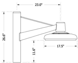
Angle Support Arm, Single (1-U02)
