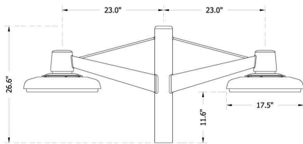
Angle Support Arm, Double (2-U02)
