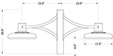
Sweep Arm Side Mount, Double (2-U01)
