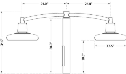
Archway Arm, Double (2-U04)
