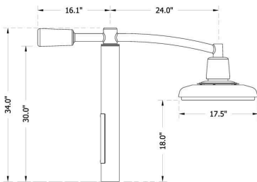
Archway Arm, Single (1-U04)
