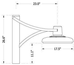
Sweep Wrap Arm, Single (1-U01S)
