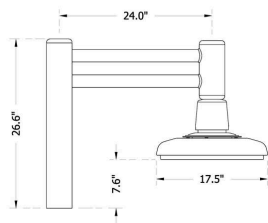
Horizontal 2 Pipe Arm, Single (1-U03)
