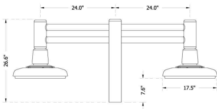
Horizontal 2 Pipe Arm, Double (2-U03)
