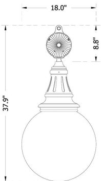
Catenary Mount (CAT) 18" Globe, "5P" Fitter
