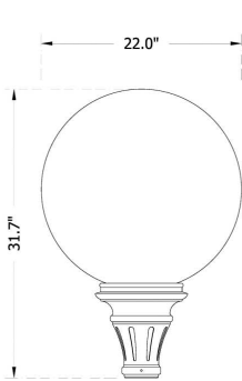
22" Globe, "5P" Fitter
