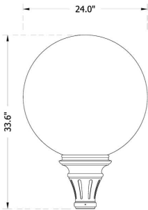
24" Globe, "5P" Fitter
