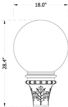
18" Globe, "OL3" Fitter
