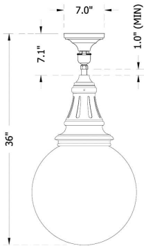
Stem Hung (SH44) 18" Globe, "5P" Fitter
