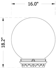
16" Globe, "C2097" Fitter
