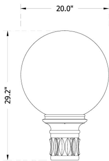
20" Globe, "BD5" Fitter
