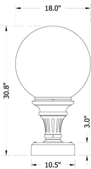
Pier Base (450PB) 18" Globe, "5P" Fitter
