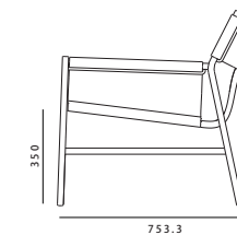
FOOTREST SIDE
