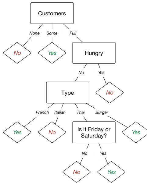
A decision tree about restaurants 1
