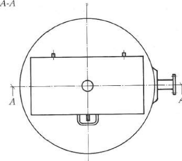
Figur V 4.4.4 a. Installationsbrønd
