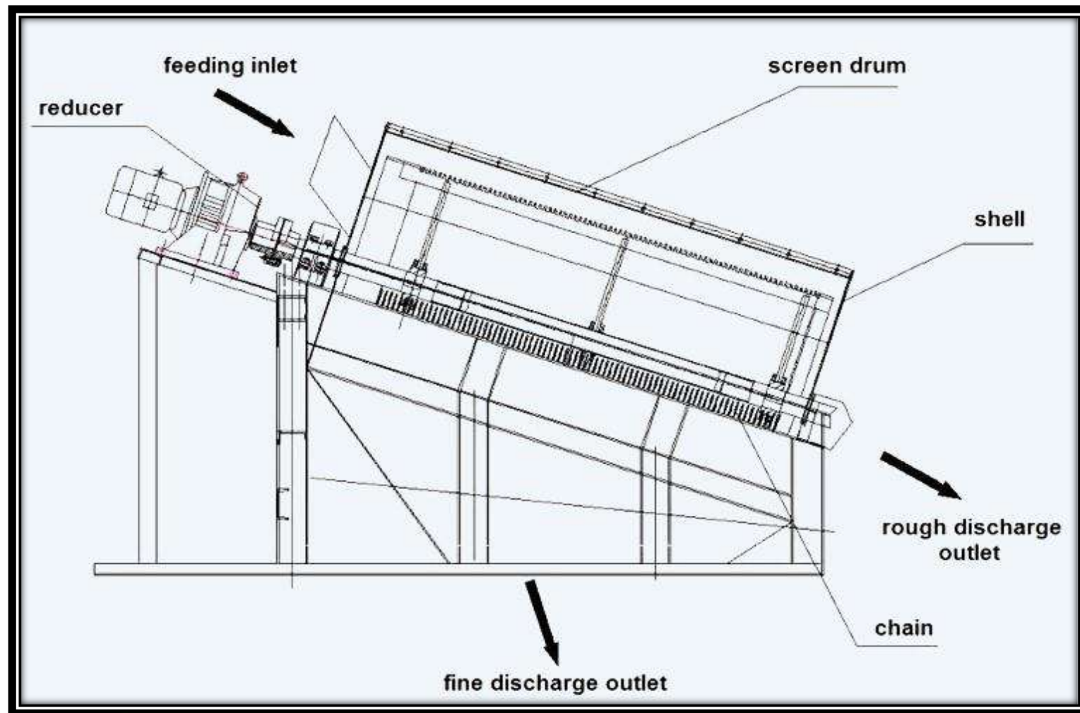
Schematic labelled diagram of a trommel screen
