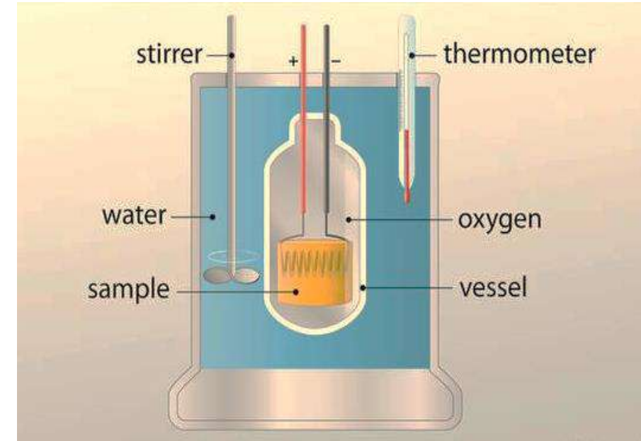
BOMB CALORIMETER
