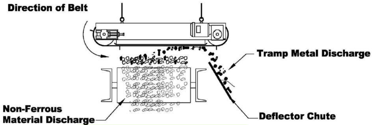
Pictorial representation of a suspended magnetic separator
