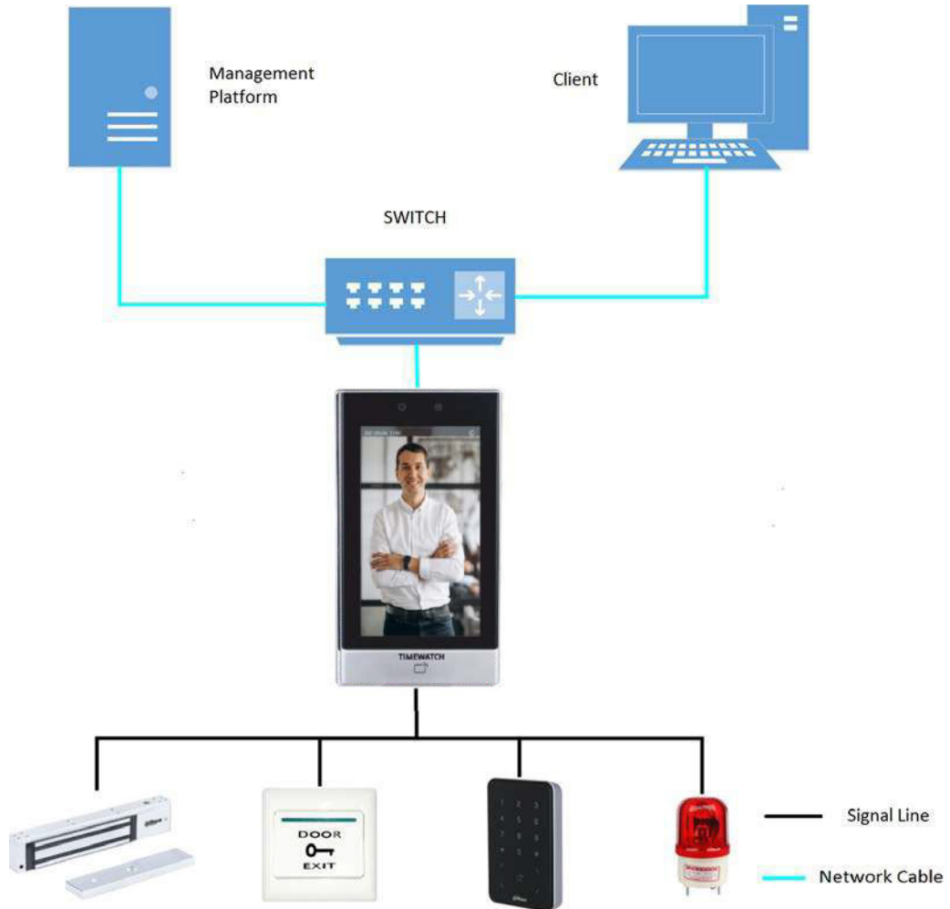
Figure 1-1 Networking
