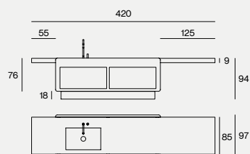
DIMENSIONS 420X97X94H
