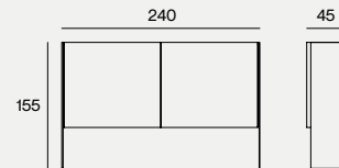
DIMENSIONS 240X45X155H
