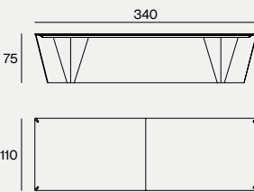
DIMENSIONS 340X110X75H
