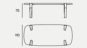
DIMENSIONS 250X110X75H
