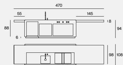
DIMENSIONS 470X108X94H
