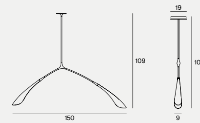
DIMENSIONS 150X19X110H
