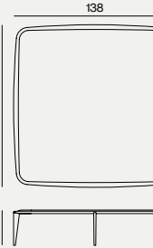
DIMENSIONS 138X138X30H
