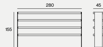
DIMENSIONS 280X45X155H
