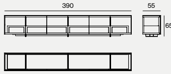
DIMENSIONS 390X55X65H
