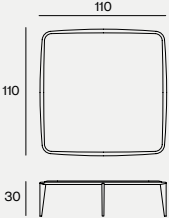
DIMENSIONS 110X110X30H
