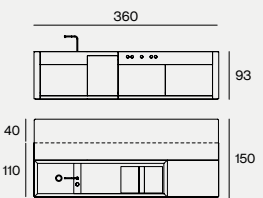
DIMENSIONS 360X150X93H
