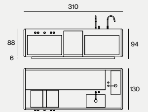
DIMENSIONS 310X130X94H
