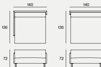
DIMENSIONS 135X140X72H
