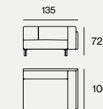
CORNER ELEMENT RH 135X100X72H
