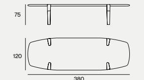
DIMENSIONS 330X120X75H
