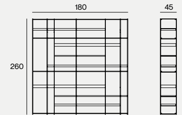
DIMENSIONS 180X45X260H
