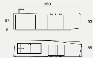
DIMENSIONS 360X85X93H
