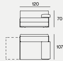
ELEMENT A WITH TRAY R 120X107X70H
