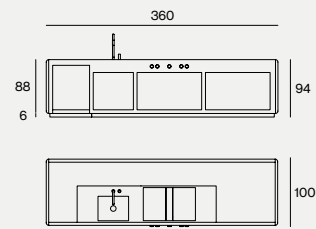
DIMENSIONS 360X100X94H
