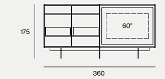
BOOKSHELF 450X40X175H
