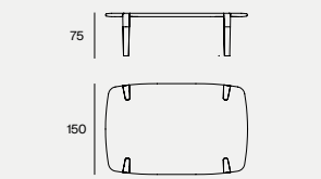
DIMENSIONS 250X150X75H
