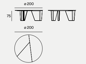
DIMENSIONS Ø 200X75H
