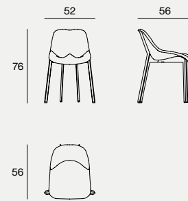
DIMENSIONS 52X57X77H
