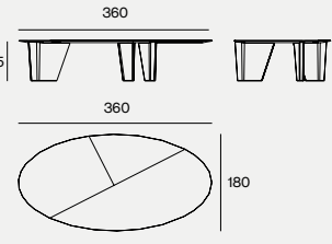
DIMENSIONS 360X180X75H
