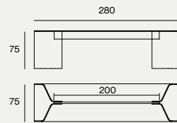
DIMENSIONS 280X75X75H
