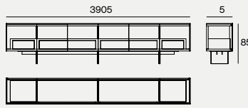
DIMENSIONS 390X55X85H
