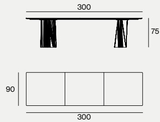
DIMENSIONS 300X90X75H
