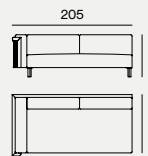
ELEMENT LH WITH WOODEN FRAME 205X100X72H
