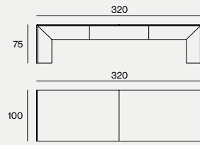
DIMENSIONS 320X100X75H
