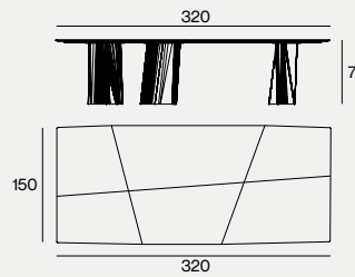
DIMENSIONS 320X150X75H
