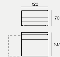
ELEMENT C WITH TRAY L 120X107X70H
