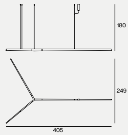
DIMENSIONS 405X249X8H - XL A MAXI
