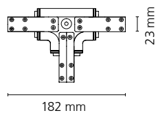
T Joint
