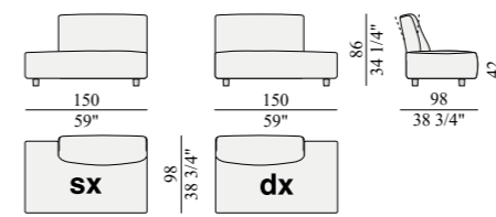
GSF150Asx GSF150Adx centrale sofa canapé Sofa
